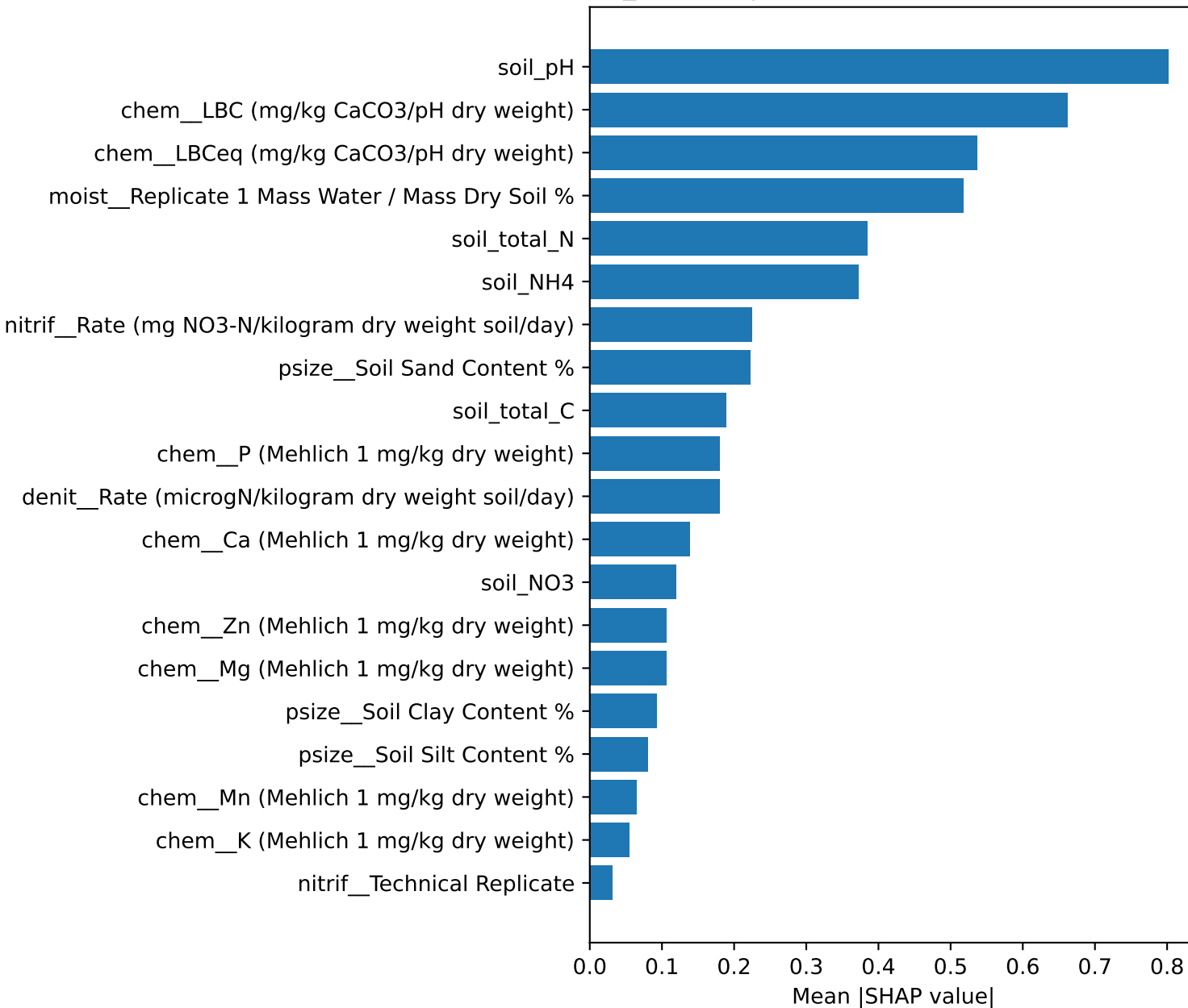
SHAP soil features C18_negative|IK:WLJVXDMOQOGPHL-UHFFFAOYSA-N Top 20 features
